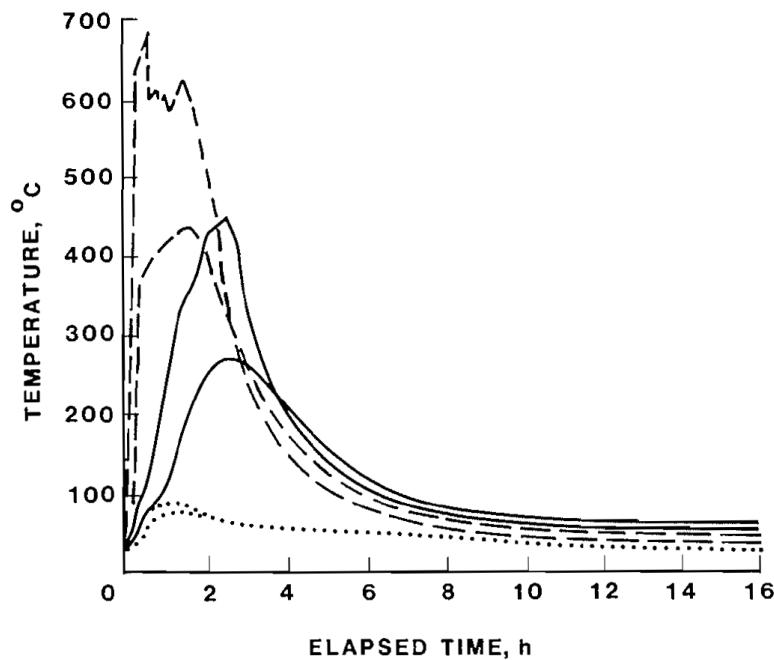
Figure 21. Temperature histories in uncovered dry sand (---), dry sand covered with wet peat moss (-), and wet sand covered with wet peat moss (···). Two curves are shown for each profile. The upper curve is the temperature at the sand surface. The lower curve is 0.8 inches (2 cm) below the surface. From Frandsen and Ryan 1986.
