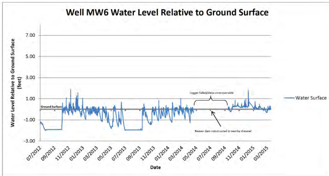
Figure 48: Data from monitoring well #6 showing a rise in the local water table following construction of a beaver dam in the nearby channel
