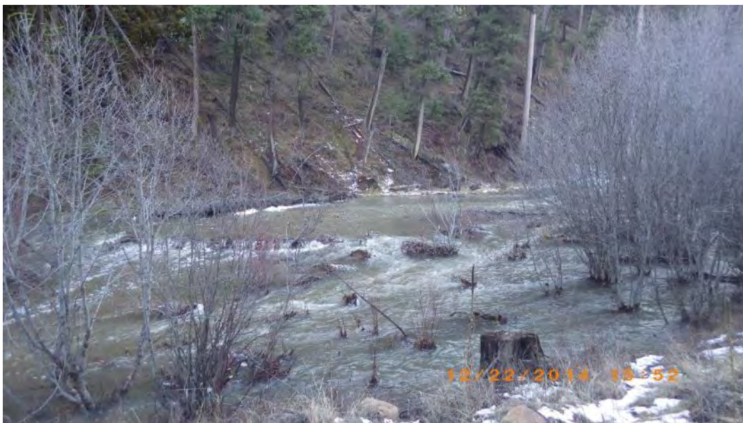
Figure 54. Valley bottom being inundated with moderate flood because of beaver dam influence (12/22/14). Same dam as Figure 52.
